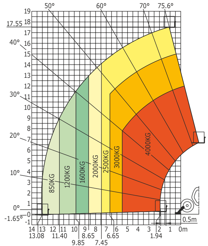
Machine on stabilizers with forks
